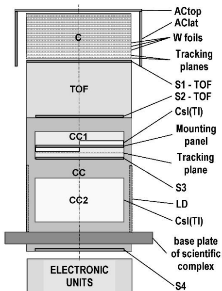
Figure 1. The physical scheme of the GAMMA-400 gamma-ray telescope.
