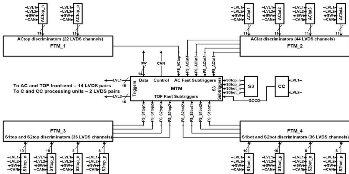
Figure 3. The functional diagram of interconnections in the frame of triggers formation cluster. The n and p postfixes designate the opposite ends of scintillation strips. FS x – “fast” subtriggers in accordance with predefined scintillation strips patterns in AC and TOF. S3 x – the signals from discriminators of S3 layers. The LVDS signal GOOD from CC main processing unit that confirms the fulfillment of predefined trigger conditions in CC1, CC2, LD, S3 and S4. SW – the high-speed SPACEWIRE network, CAN – Controller Area Network internal bus for control of front-end units.
